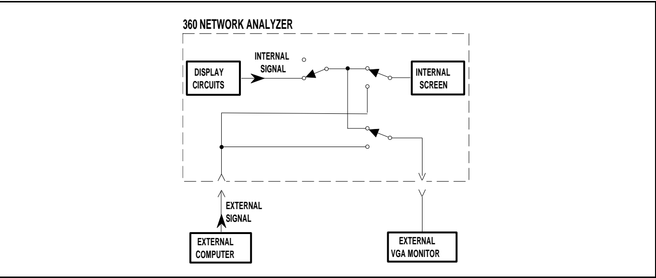
Figure 3-2. 360 VNA Video Signal Paths
